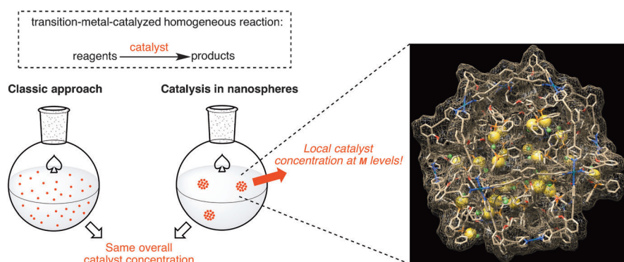
Figure 1. New approach allowing the use of high local catalyst concentration (1 M), whereas the average catalyst concentration is in the usual 10^{-3} – 10^{-6} M range.
