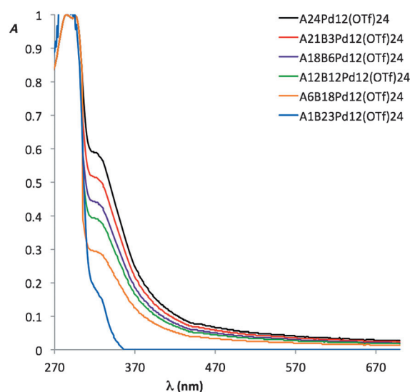
Figure 6. Normalized UV/Vis spectra of solutions of A n B 24-n Pd 12 (OTf) 24 in acetonitrile at room temperature showing an increased band at \lambda = 315 nm, indicative of d 10 –d 10 aurophilic interactions at high local concentrations.
